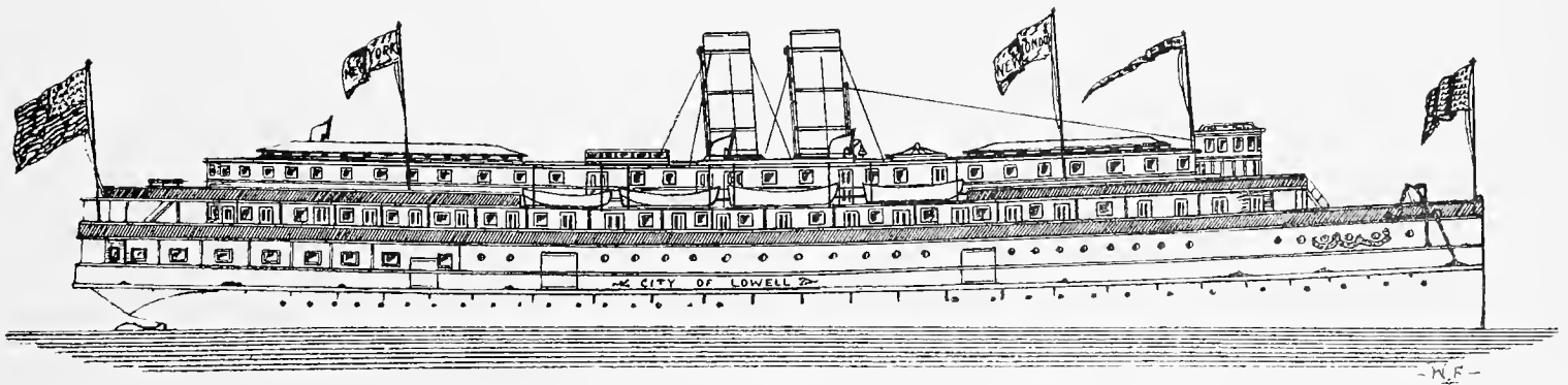
THE NORWICH LINE'S STEEL TWIN-SCREW PASSENGER STEAMER CITY OF LOWELL. Built by the Bath (Maine) Iron Works from Plans of A. Cary Smith.
